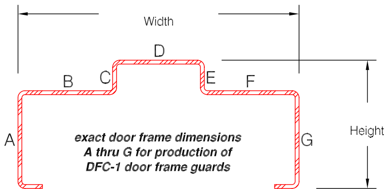
Frame Dimensioning Detail
