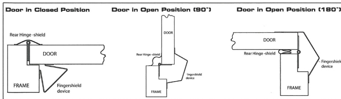
FG3 Full door set
